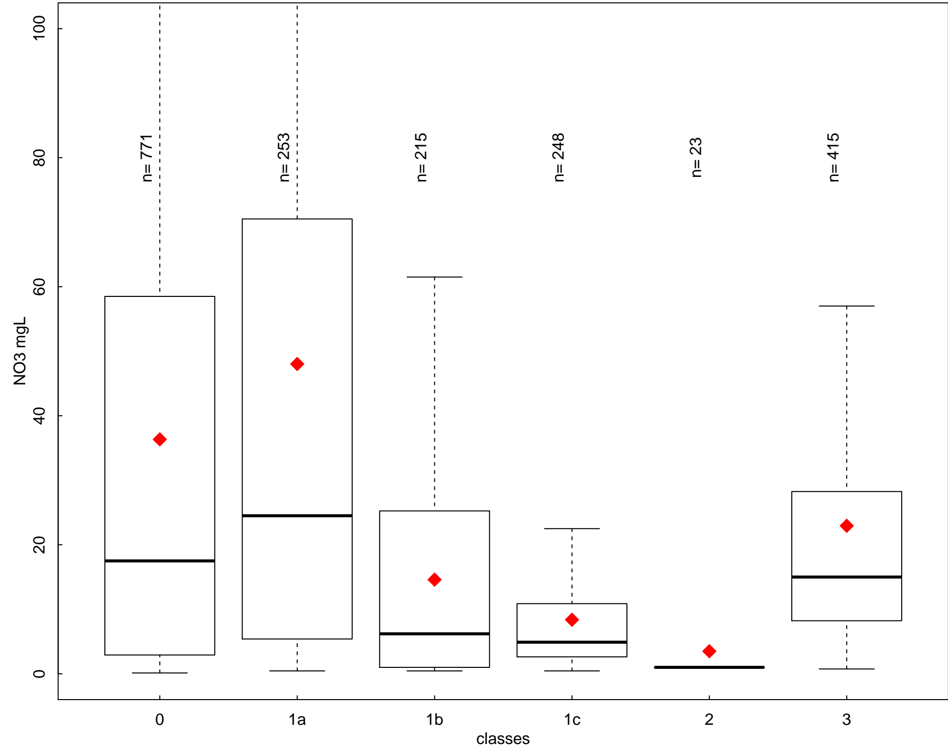
Annual NO3 (mgL) by class type- period 2012-2015 - PT
