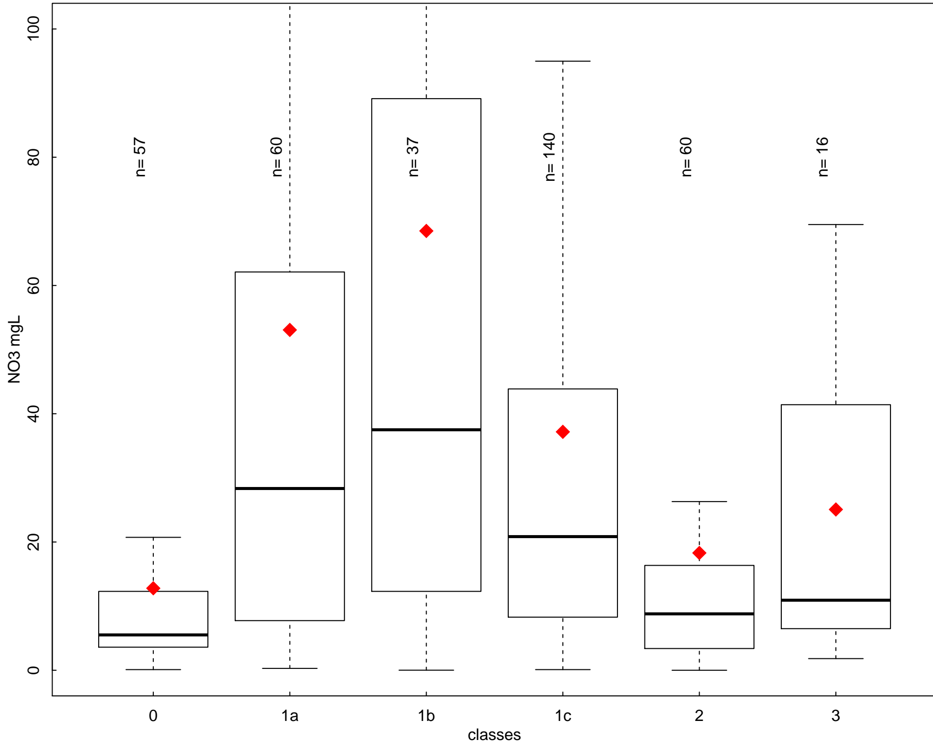
Annual NO3 (mgL) by class type- period 2008-2011 - GR
