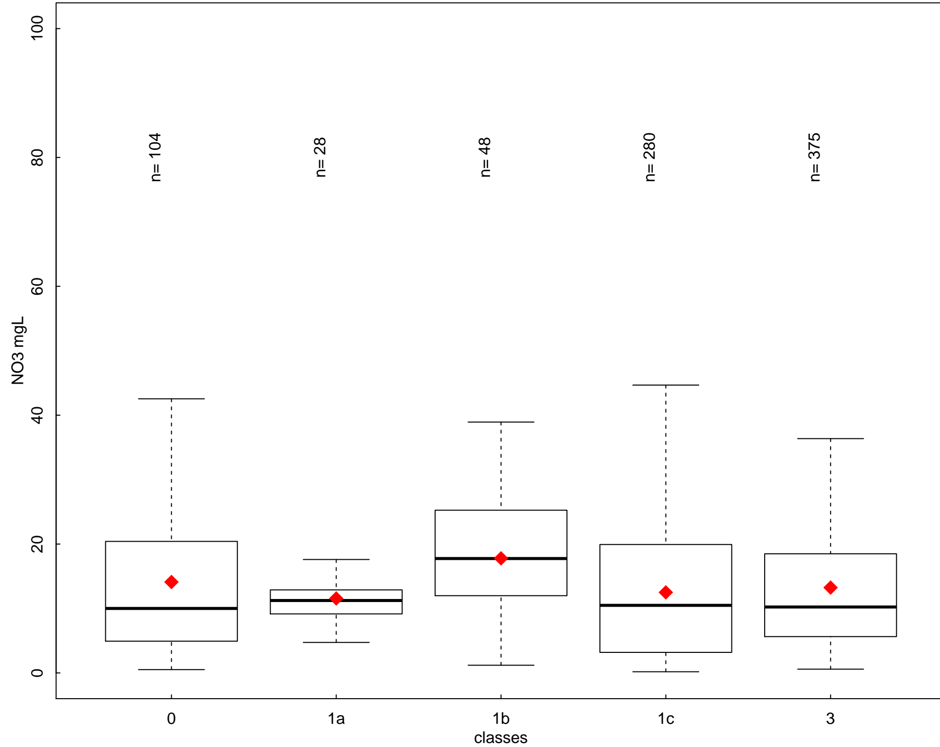
Annual NO3 (mgL) by class type- period 2008-2011 - IE
