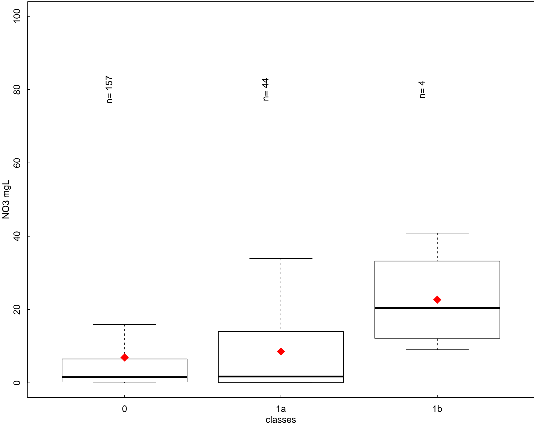
Annual NO3 (mgL) by class type- period 2008-2011 - LT
