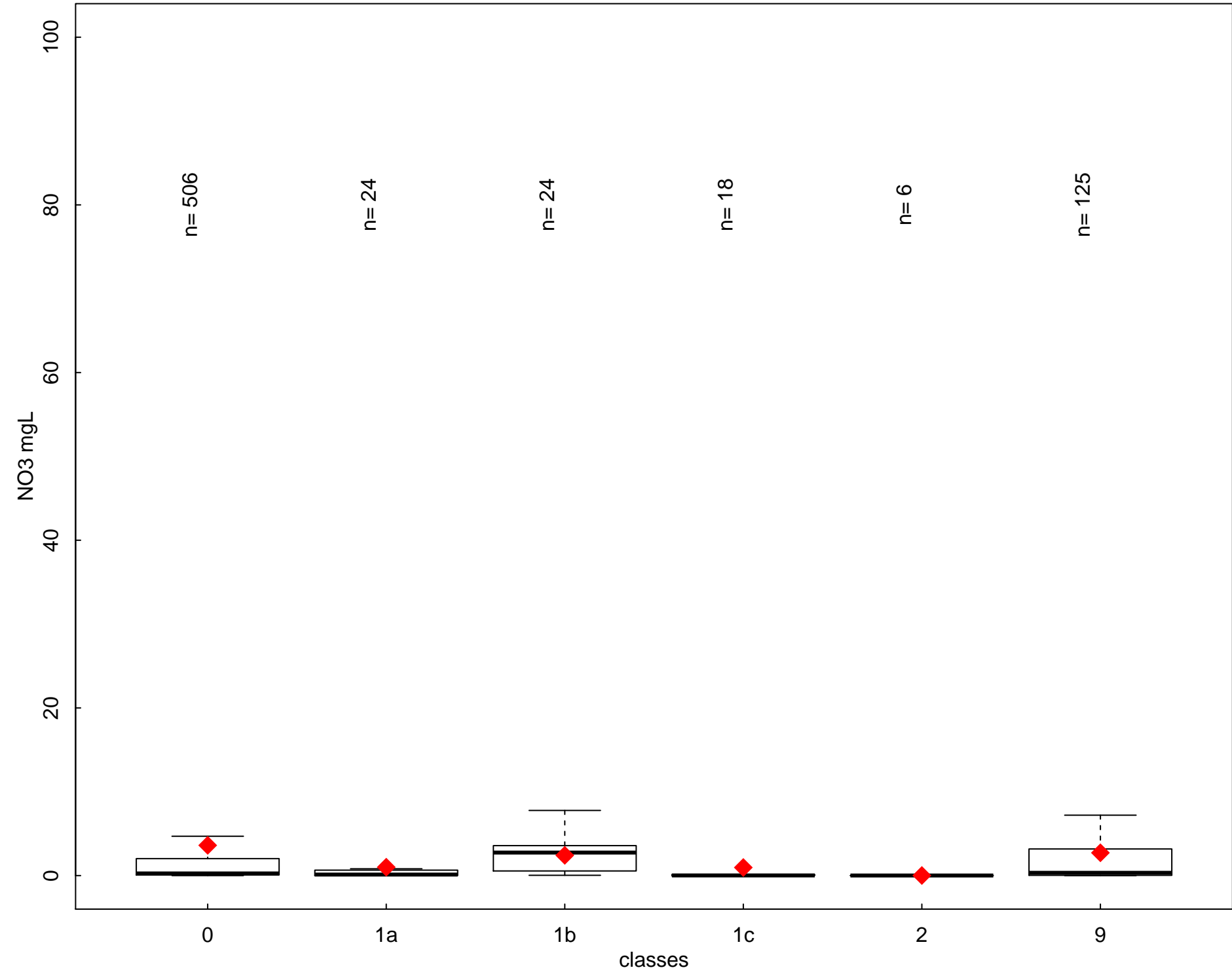
Annual NO3 (mgL) by class type- period 2012-2015 - SE
