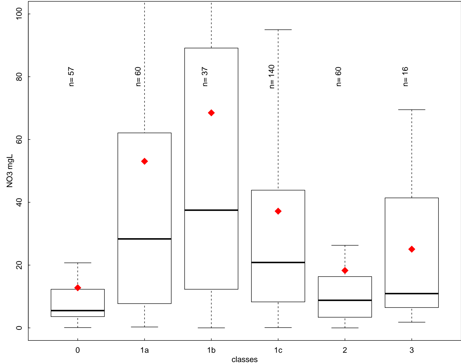
Annual NO3 (mgL) by class type- period 2008-2011 - HR
