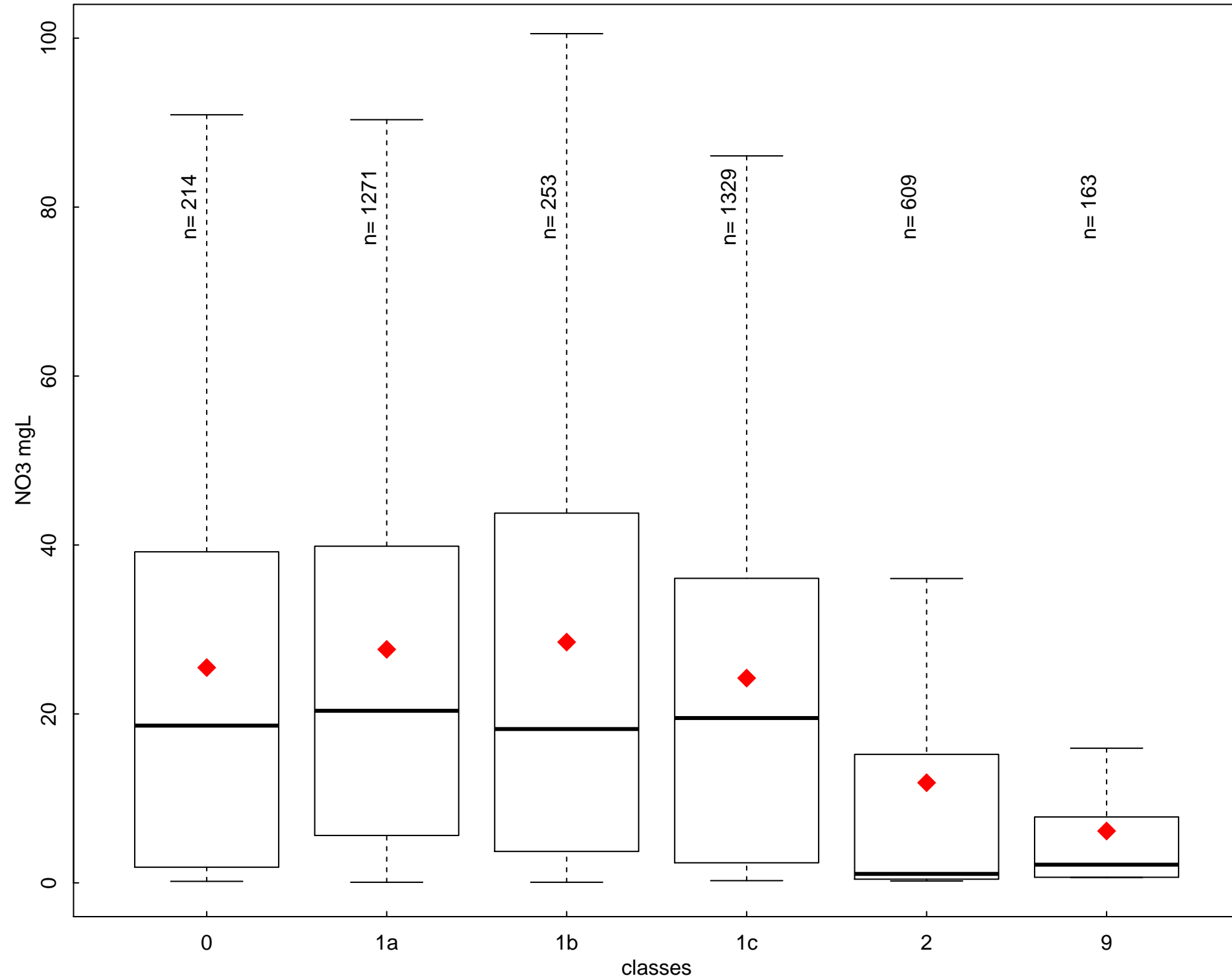
Annual NO3 (mgL) by class type- period 2008-2011 - GB
