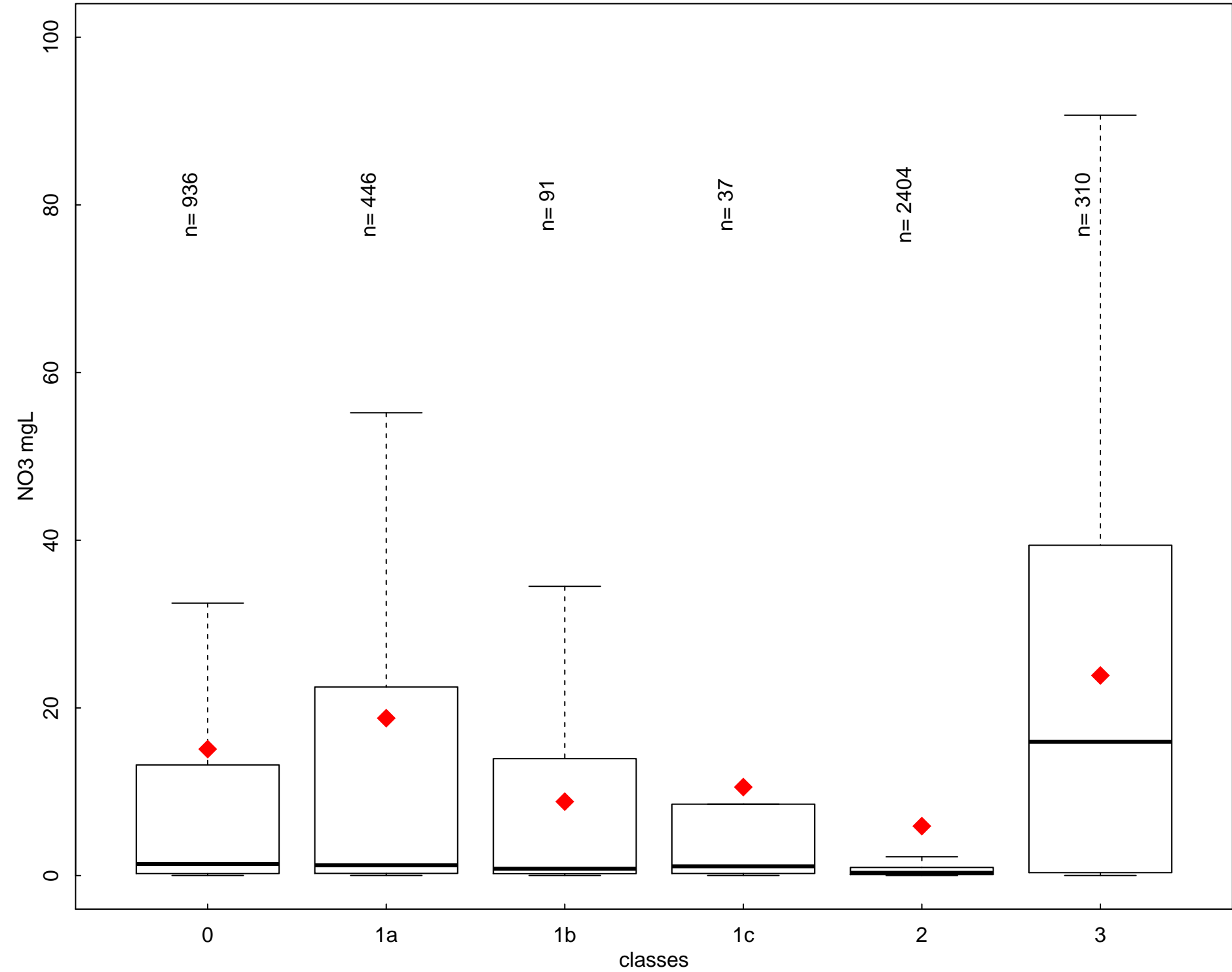
Annual NO3 (mgL) by class type- period 2012-2015 - PL
