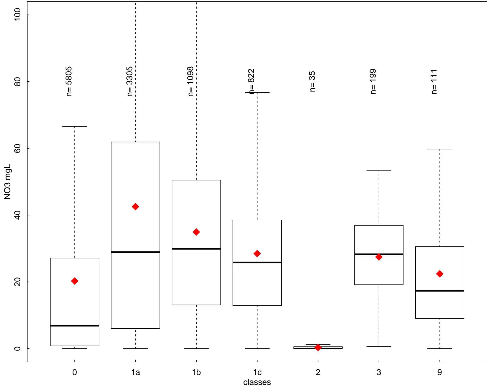
Annual NO3 (mgL) by class type- period 2008-2011 - BE
