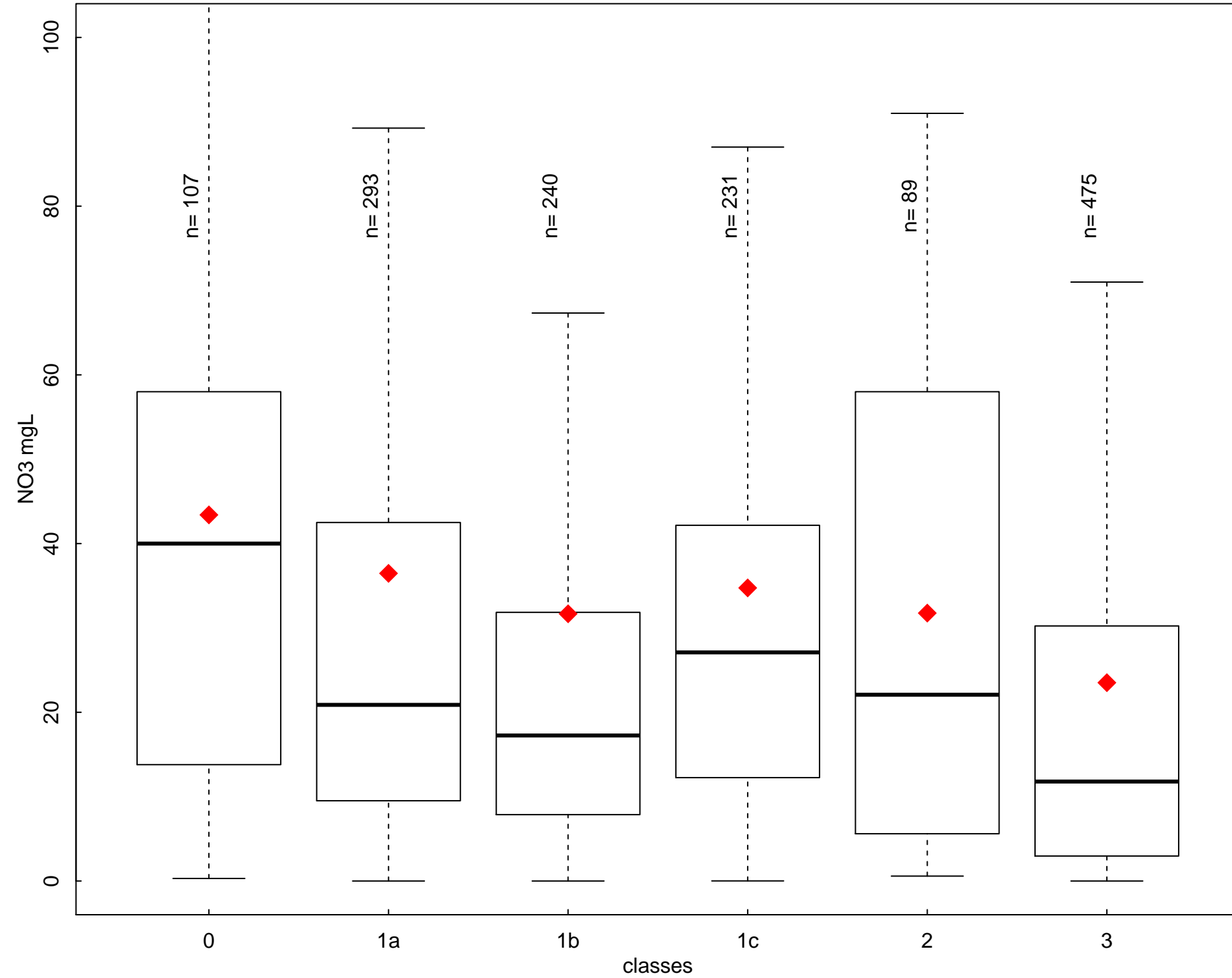
Annual NO3 (mgL) by class type- period 2012-2015 - BG
