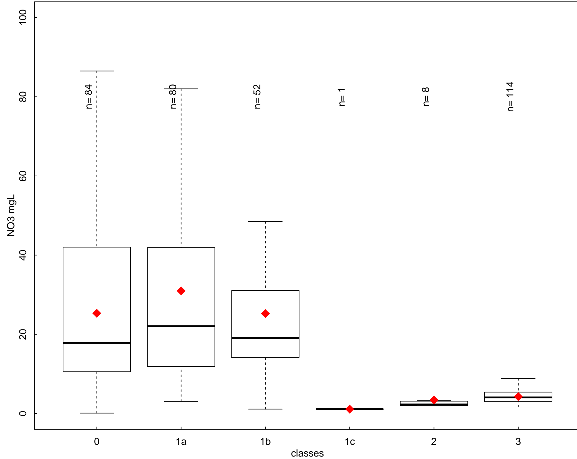
Annual NO3 (mgL) by class type- period 2008-2011 - SI
