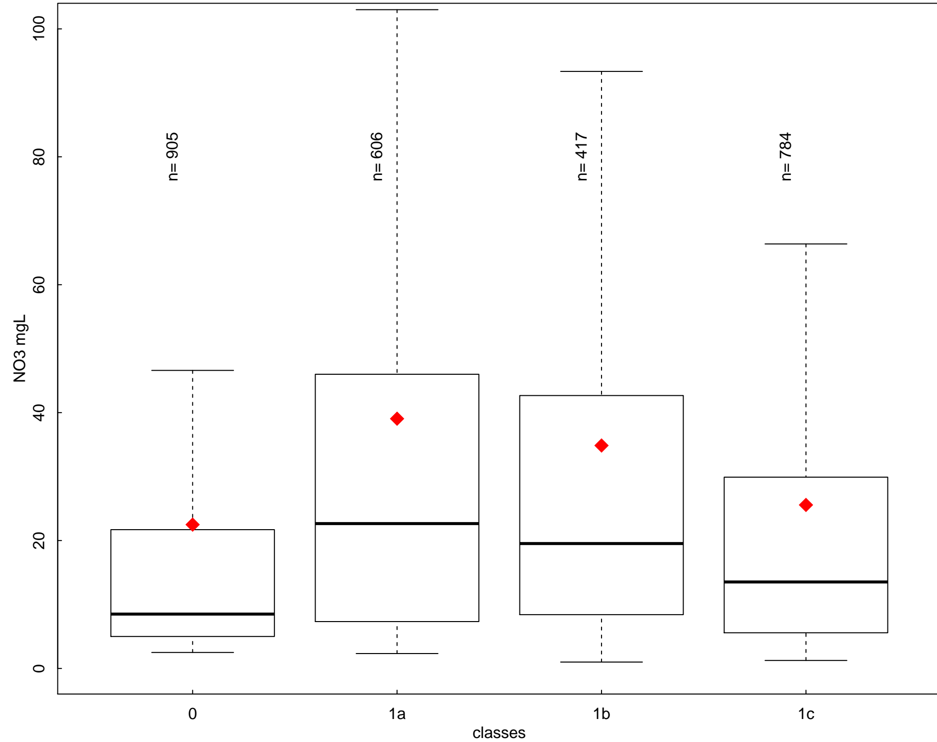
Annual NO3 (mgL) by class type- period 2012-2015 - GR
