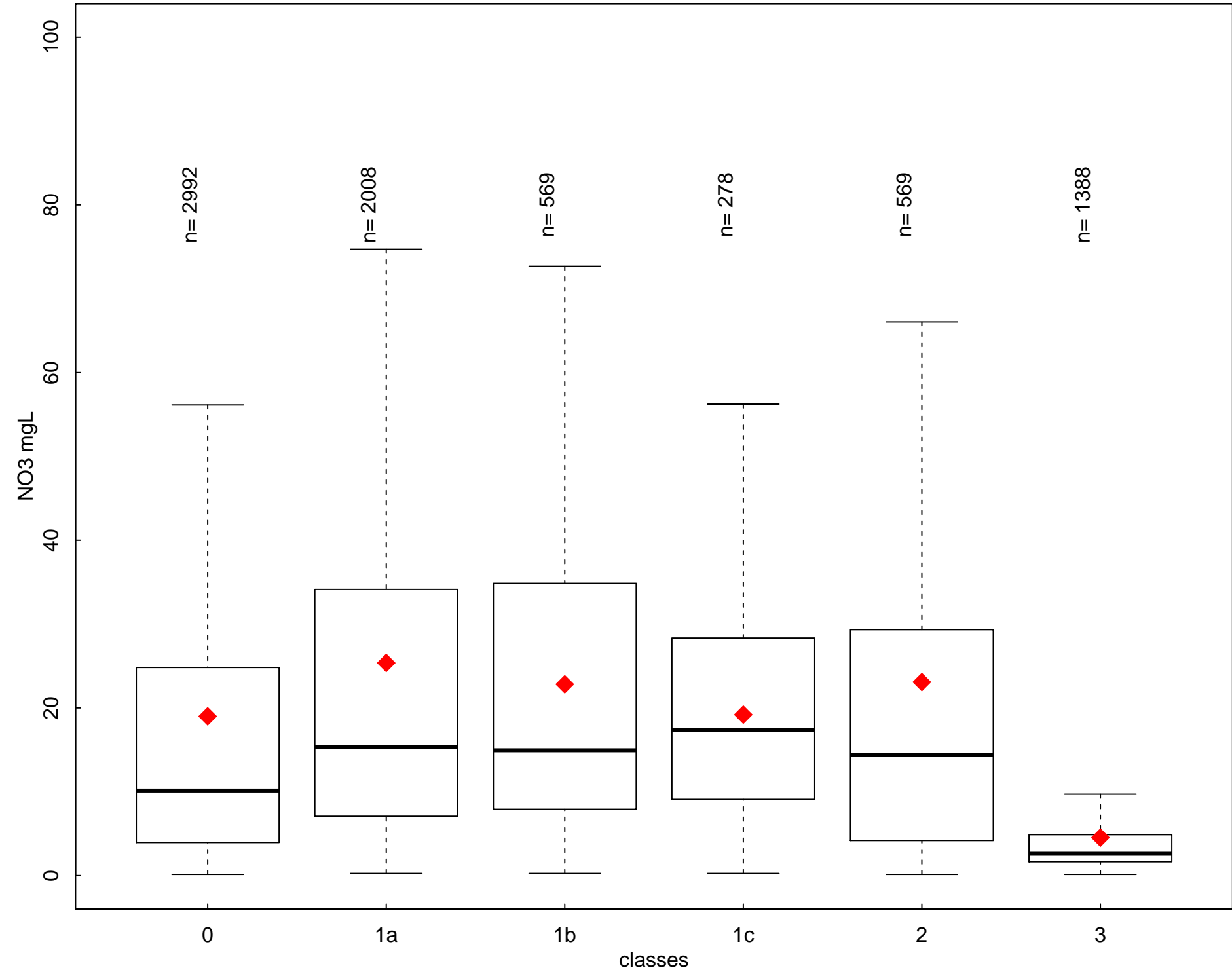
Annual NO3 (mgL) by class type- period 2012-2015 - AT
