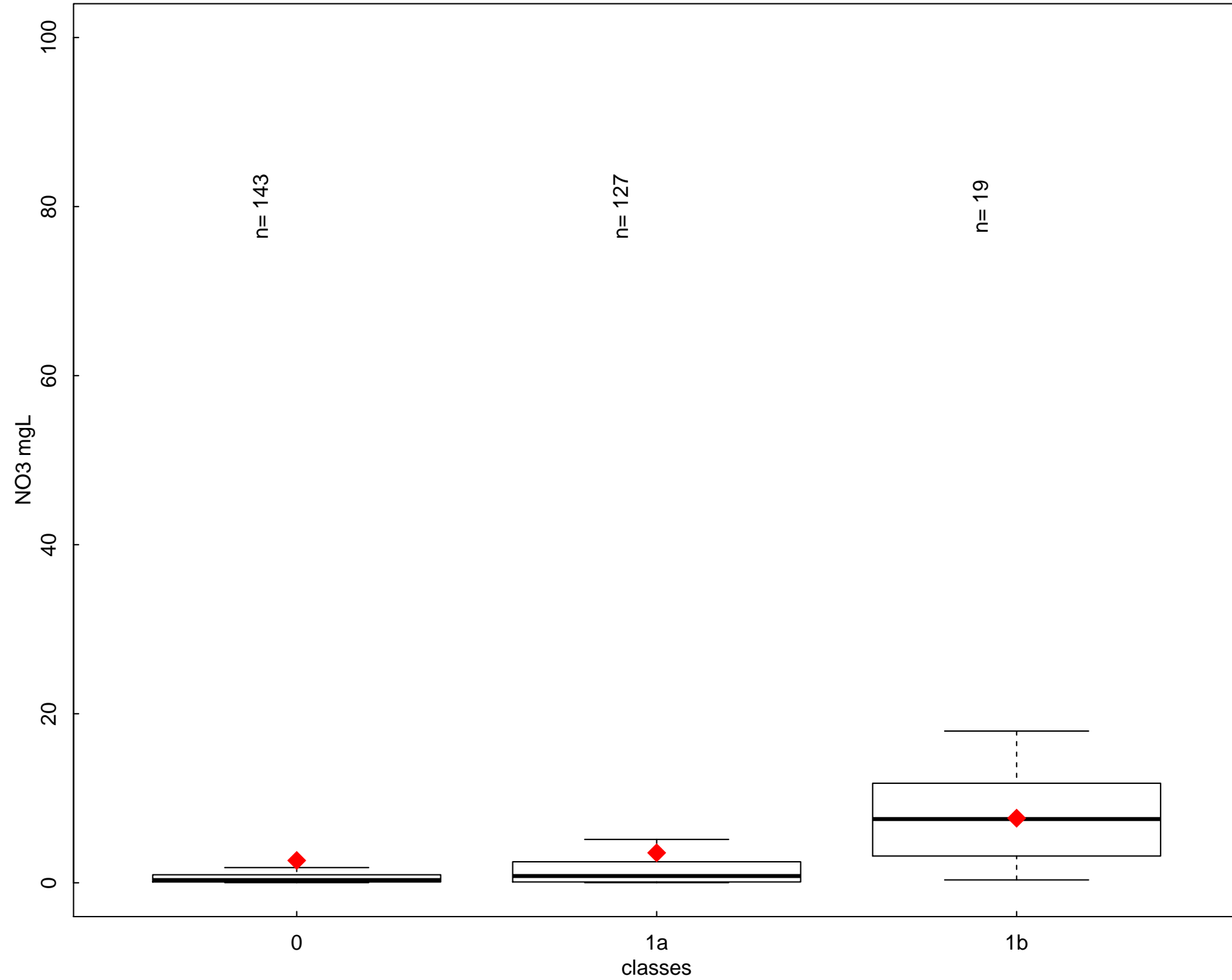
Annual NO3 (mgL) by class type- period 2008-2011 - FI
