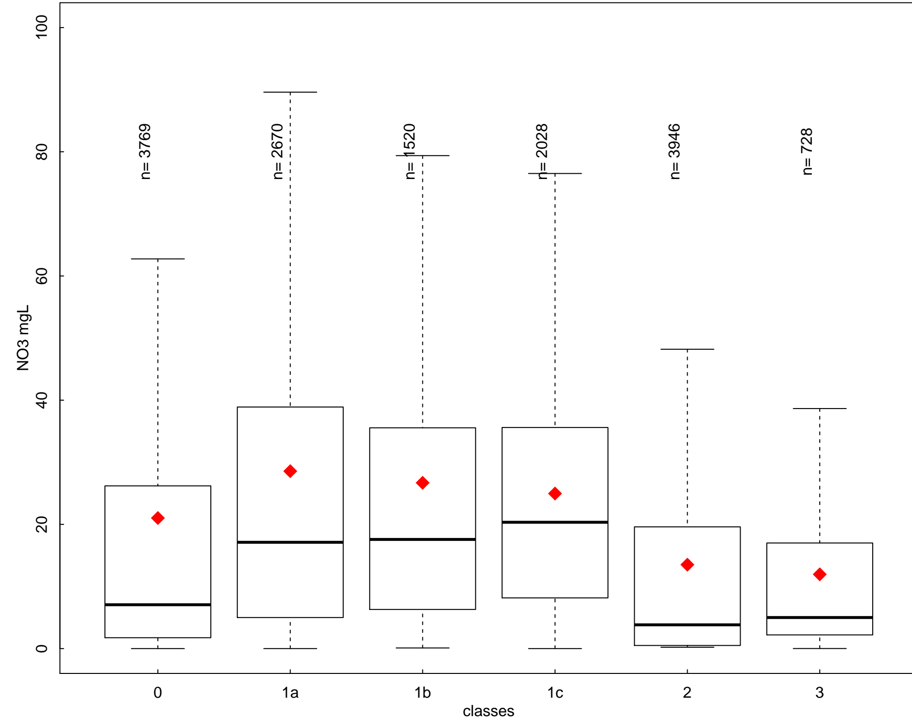
Annual NO3 (mgL) by class type- period 2012-2015 - IT
