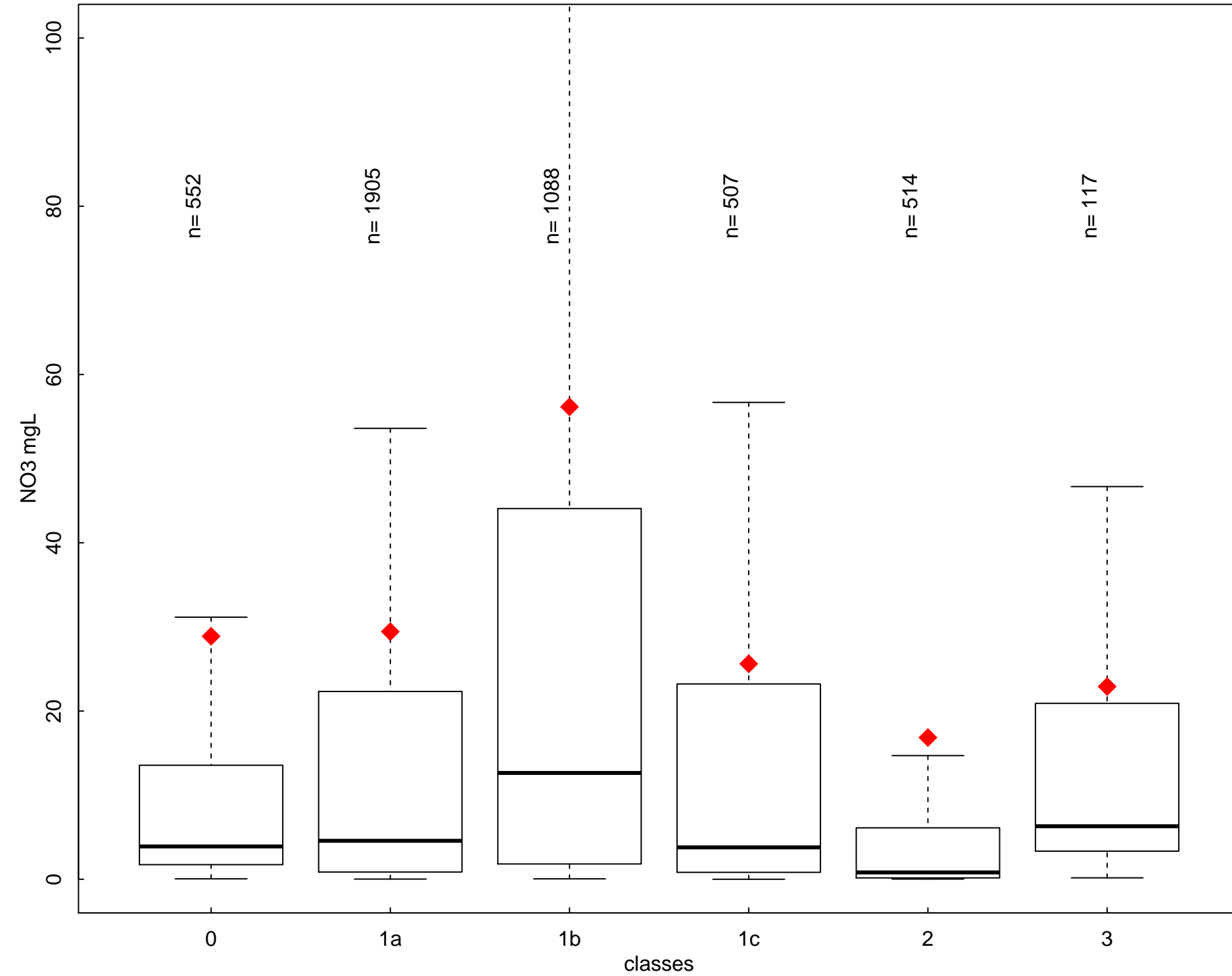
Annual NO3 (mgL) by class type- period 2012-2015 - RO
