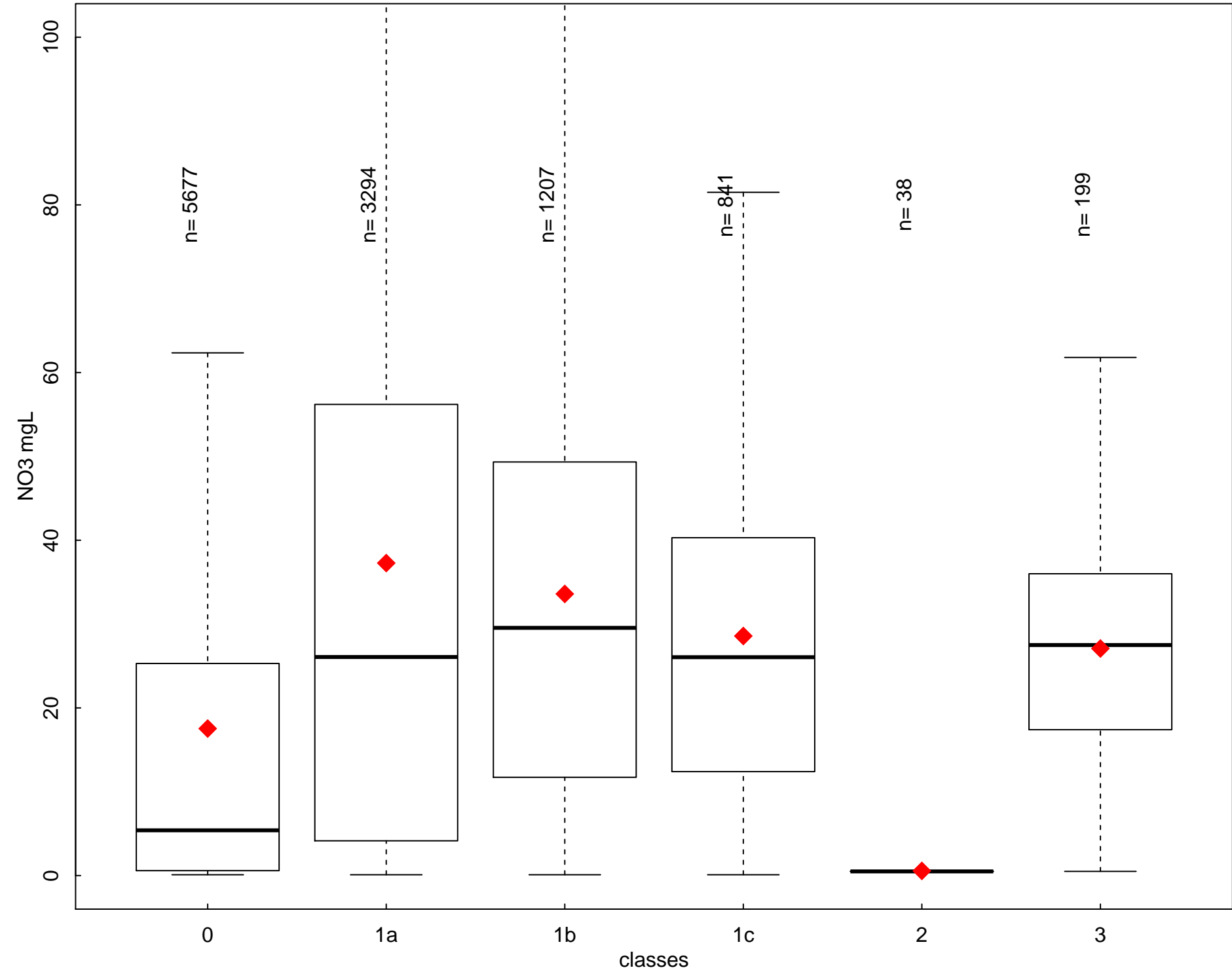
Annual NO3 (mgL) by class type- period 2012-2015 - BE
