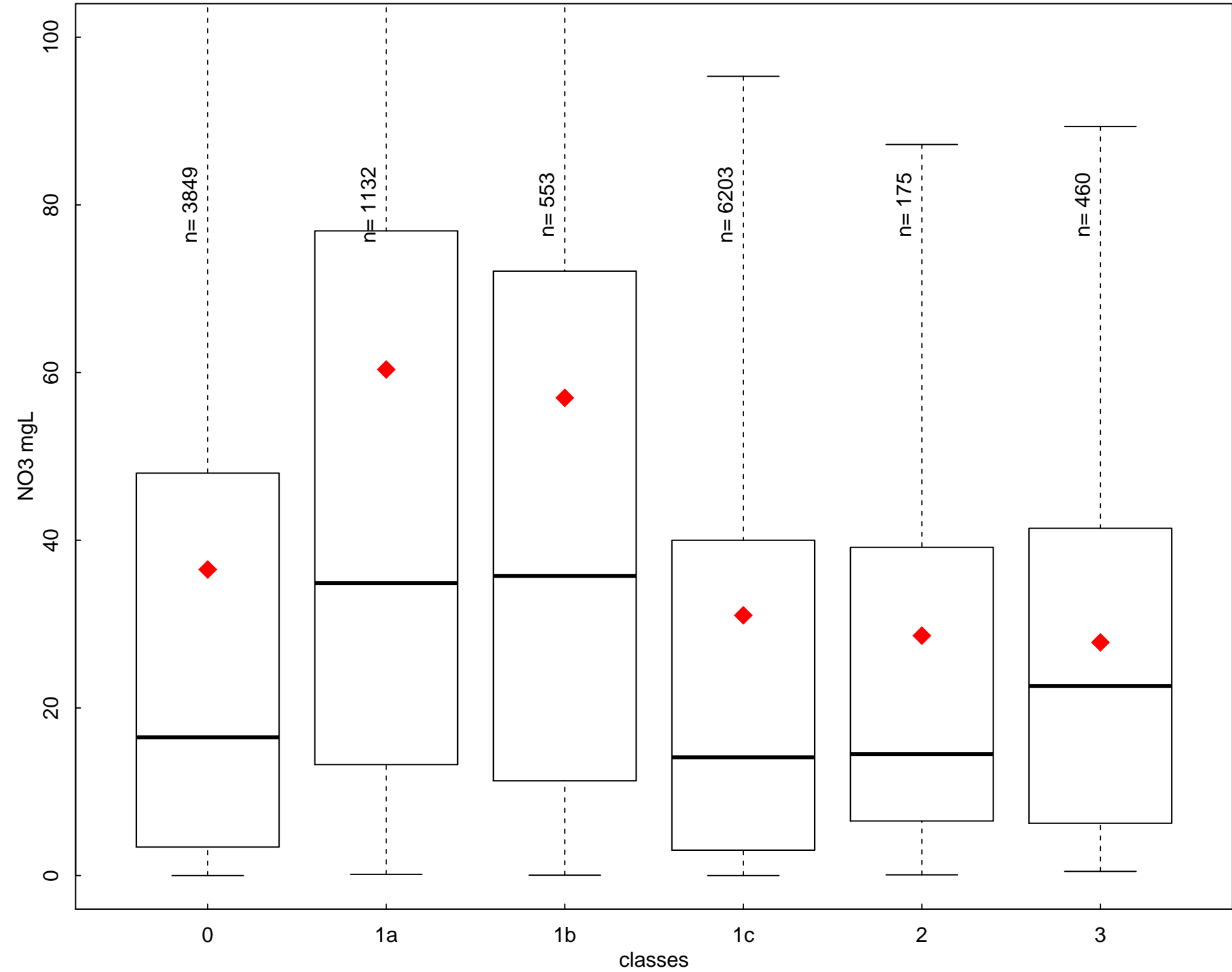
Annual NO3 (mgL) by class type- period 2012-2015 - ES
