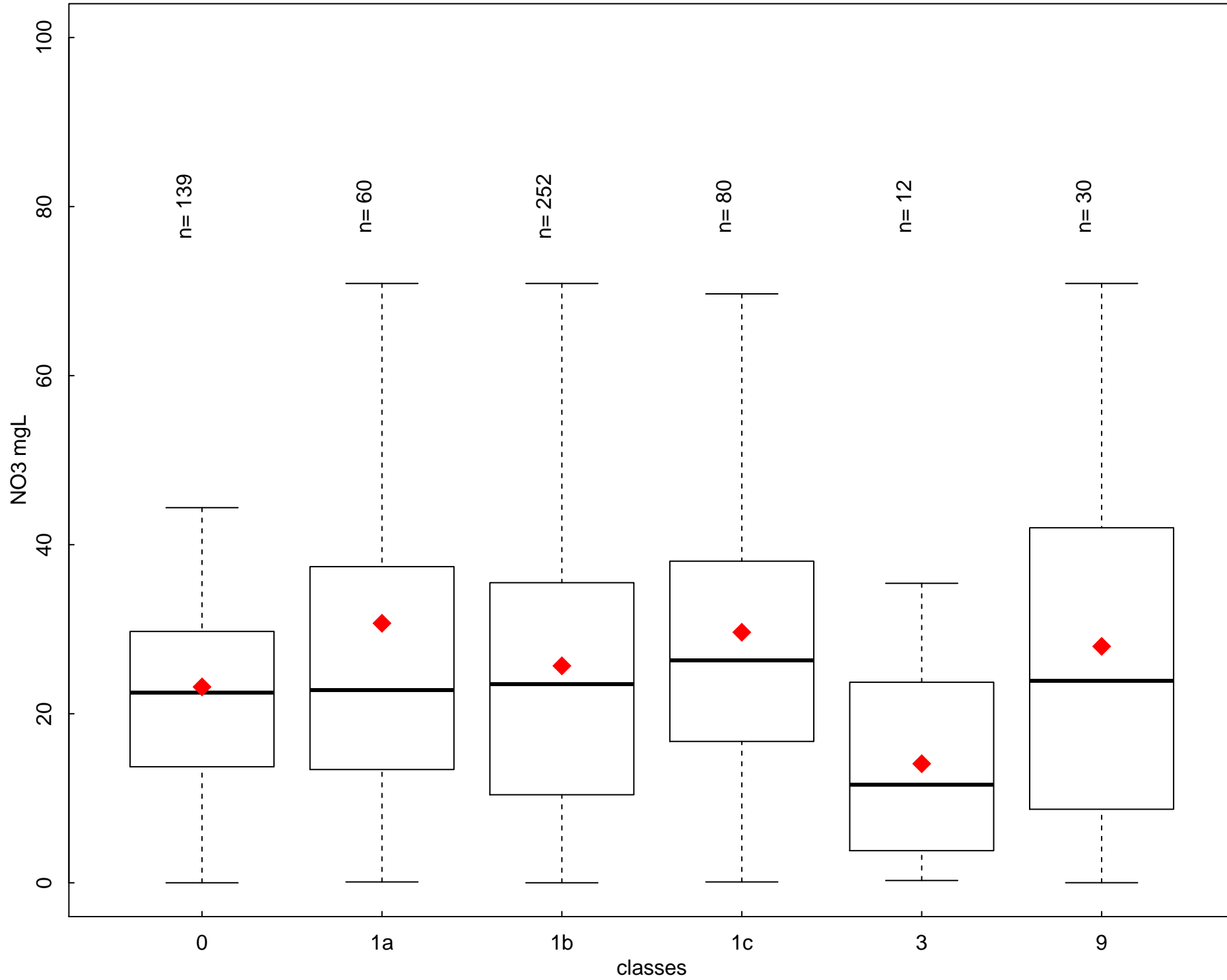
Annual NO3 (mgL) by class type- period 2008-2011 - EE
