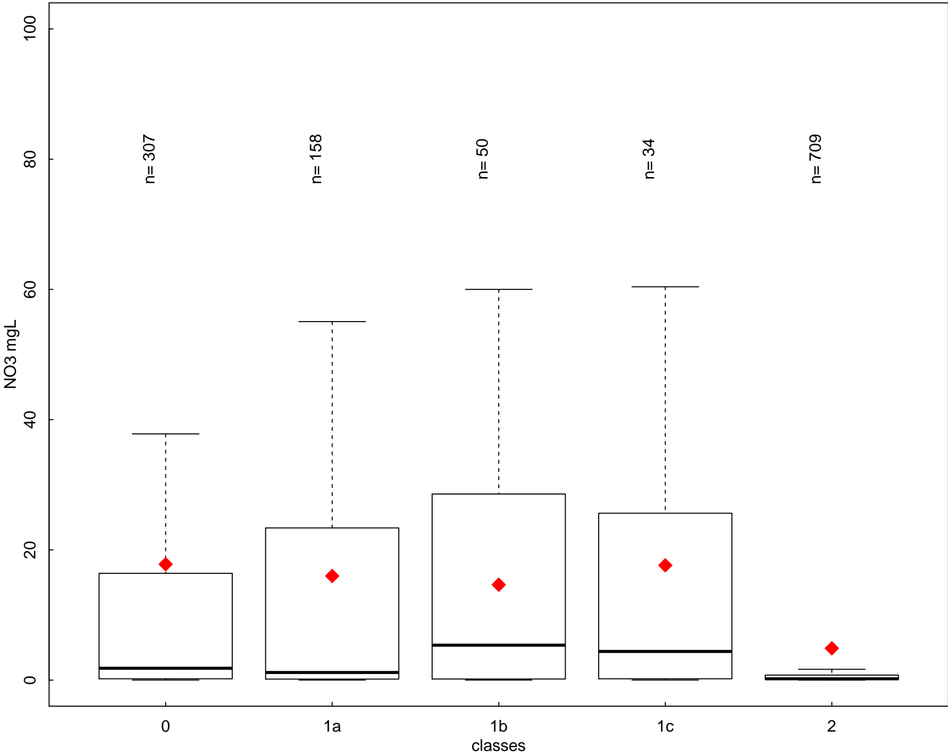
Annual NO3 (mgL) by class type- period 2008-2011 - PL
