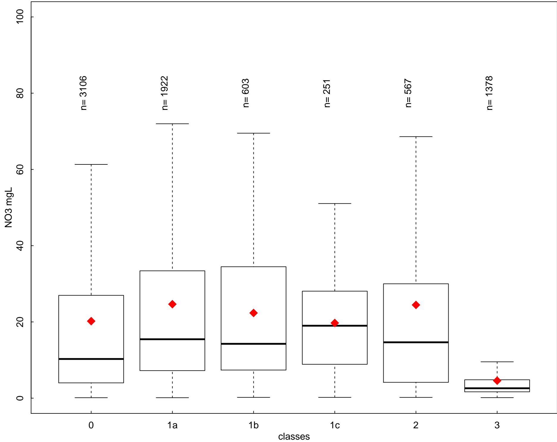
Annual NO3 (mgL) by class type- period 2008-2011 - AT
