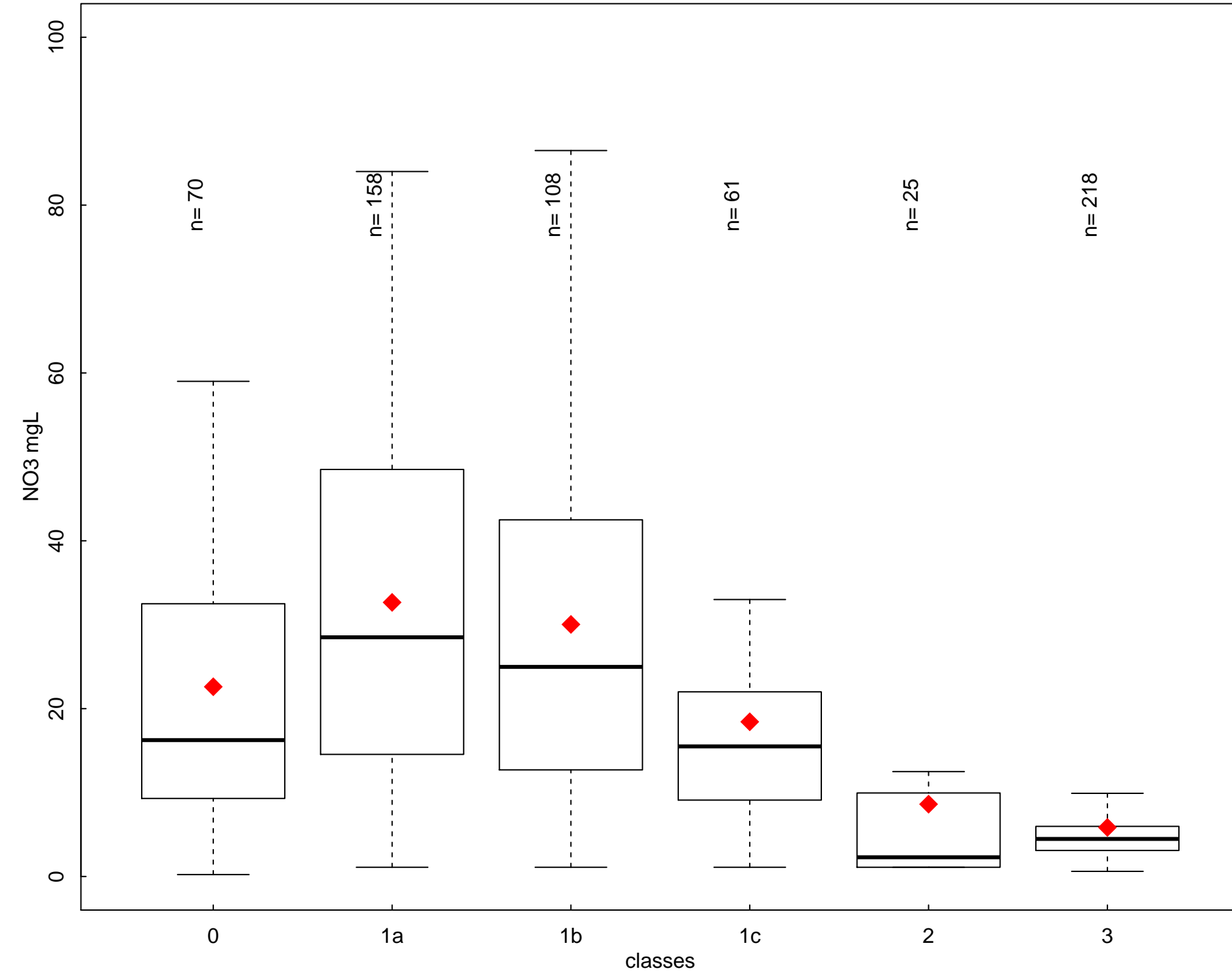
Annual NO3 (mgL) by class type- period 2012-2015 - SI
